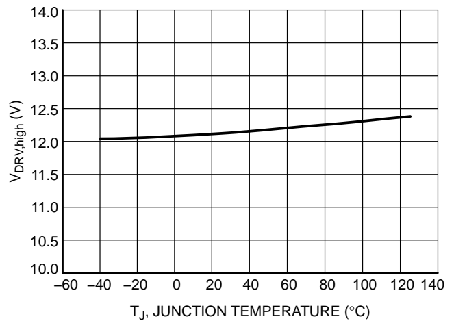
Figure 26. DRV Pin Level @ V CC = 30 V (R L = 33 kΩ & C L = 1 nF) (V DRV,high ) vs. Junction Temperature
